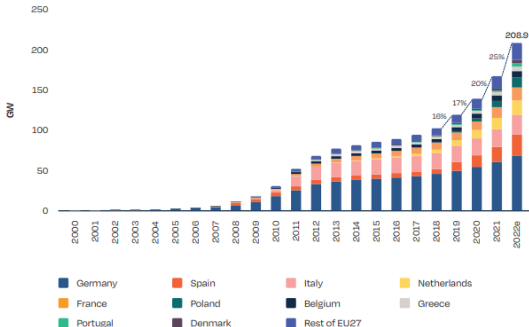
FIGURE 4 EU27 CUMULATIVE SOLAR PV INSTALLED CAPACITY 2000-2022
